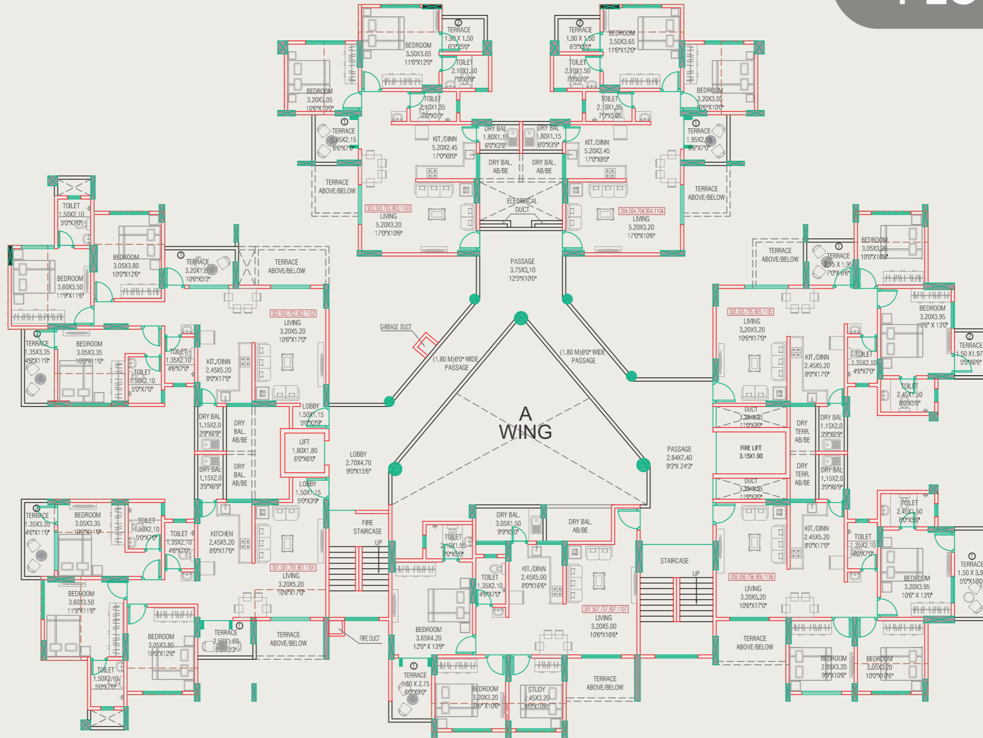
3 RD,5TH,7TH,9TH & 11TH FLOOR PLAN
